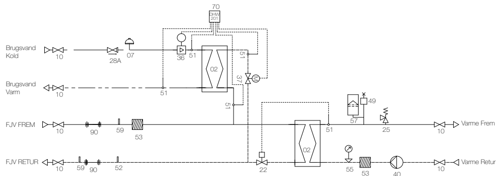
Principdiagram, Calefa V unit
